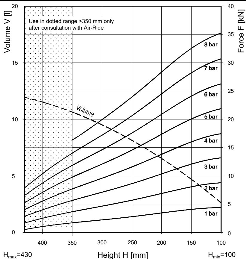
Force-height diagram
